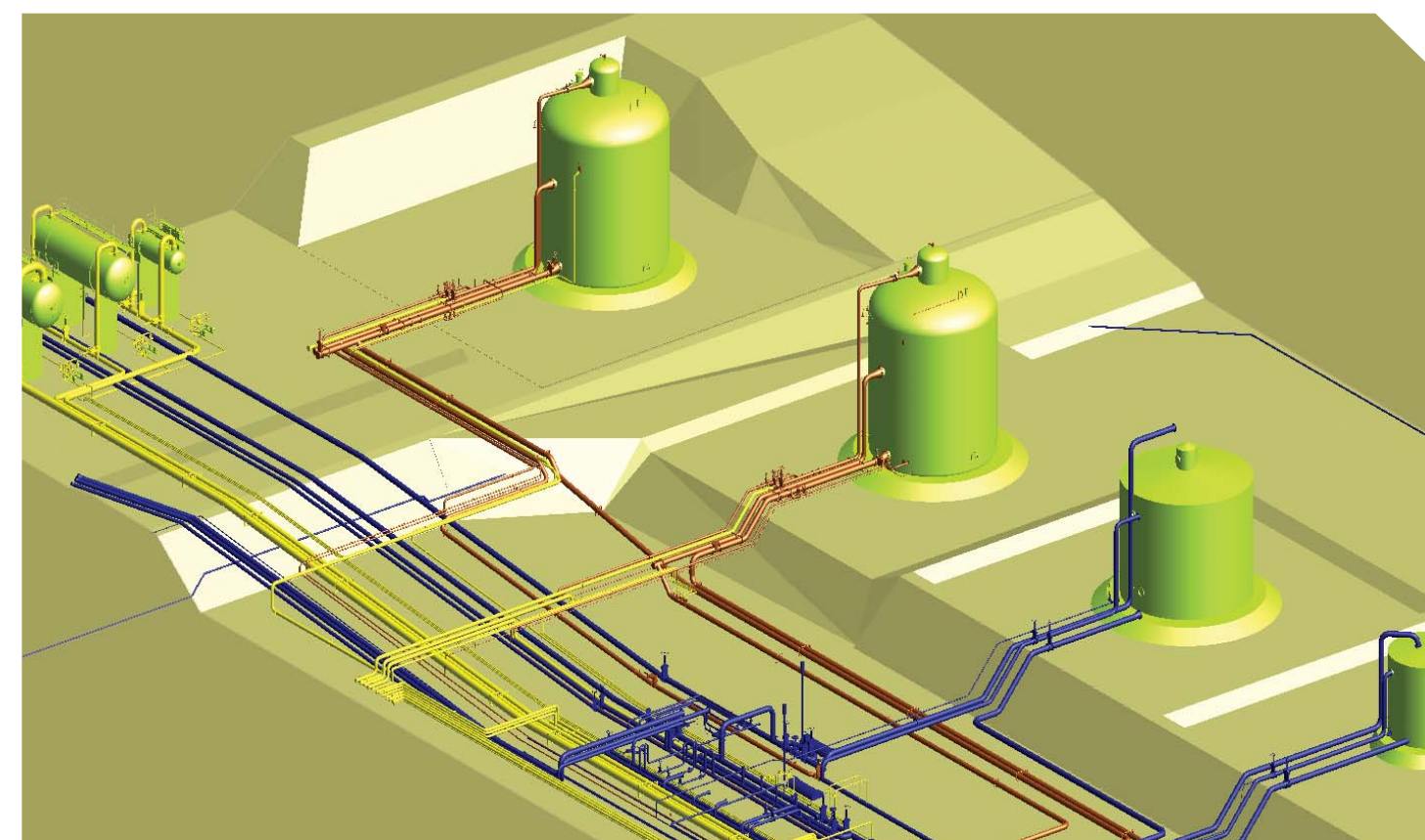
Cheshmehkhosh Surface Facility
